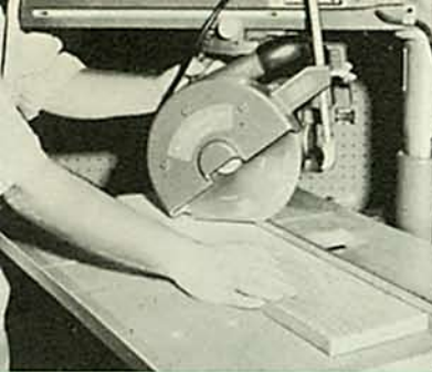
LEFT-HAND MITER. By turning saw 180° to opposite side, difficult left-hand miters are accomplished in the middle of the work table—easily, perfectly.
