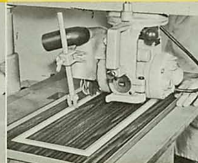
PANEL SINKING. Lower the dado \frac{1}{8} inch and make cuts illustrated by pushing stock.
