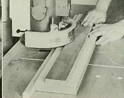
RABBET-CUT. By taking advantage of the dado diameter, you can make wide-width rabbet cuts with amazing ease and speed!
