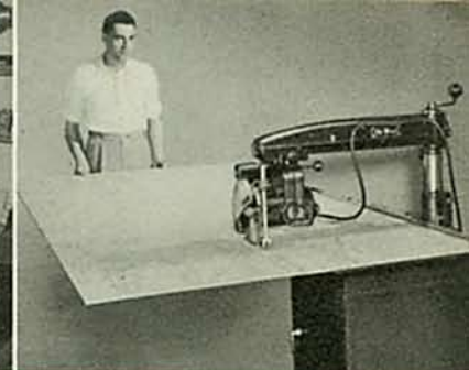
WIDE-PANEL RIPPING. The new DE WALT Power Shop rips to the center of large, standard 4 ft. wide plywood sheets. All this and accuracy, too!
