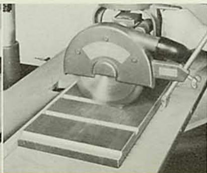
PARALLEL DADO. Almost impossible to accomplish with any accuracy on old-type saws. You must see what you're doing. DE WALT lets you!
