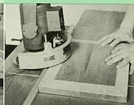
RAISED PANELS. An easy way to make expensive mill-work for your panelled walls, cabinet doors, and special drawer fronts!
