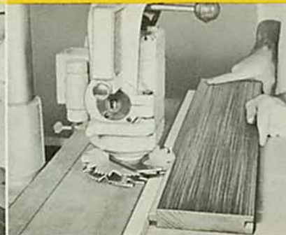
TONGUE AND GROOVE. Make your own flooring, wood panels, etc., simply by using dado inserts with collars to exact dimension needed. Tool Guard removed to show cut.
