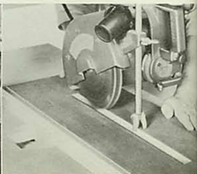
CENTER PLOUGHING. This cut is made by lowering dado into your material and raising it at the end of cut.
