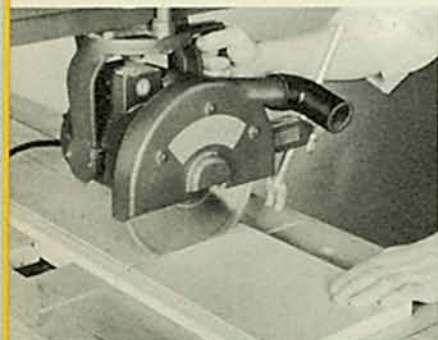
CROSS-CUT. You'll think it's magic when you cut a perfect 90° cross-cut with only one arm motion!
