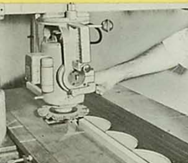
SCALLOPING. Feed the stock against the dado as shown and put unusual scallop design on your window valances. Tool Guard removed to show cut.
