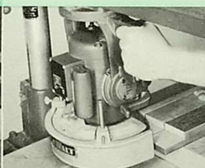
LAP JOINT CUT
