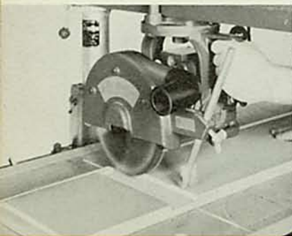
CROSS DADO. For fitting ends of shelves into sides of bookcases—and countless other uses!
