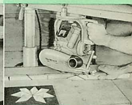
DIAMOND SHAPES. After bevel ripping stock into "V" strips, set motor at 45° R. H. miter and 45° bevel. Makes beautiful decorative patterns.
