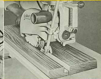
RIP AND PLOUGH. Mount saw and dado head on arbor and put into rip position. Lower for depth desired and do both cuts in single operation.
