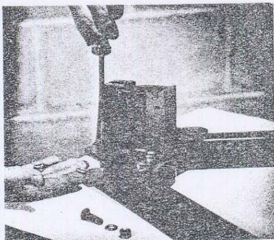
4. Assemble table frame (2 large channel pieces) to the base using (4) flat head 3/8" dia. screws, lock washers and 3/8" dia. nuts. Tighten securely with wrench. See page 26.
