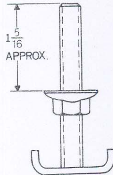
6. Screw (4) large flange hex nuts onto the threaded studs of the table cleats so the studs extend beyond the nuts approximately 1-5/16".
